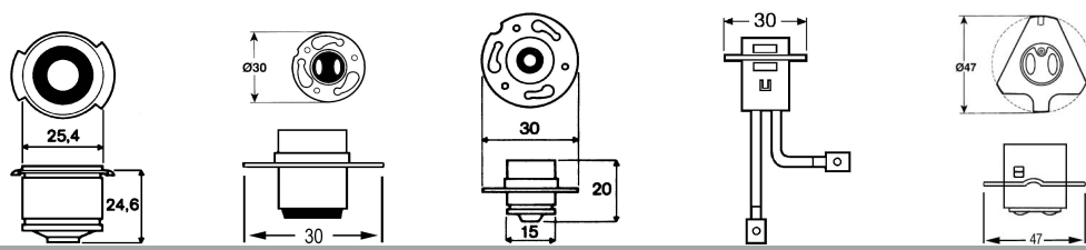
P28s P30d P30s Pk30d P47d
