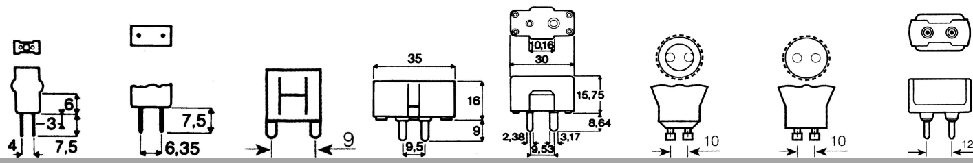
G4 G6,35-GY6,35 G9 GX9,5 GY9,5-GZ9,5 GU10 GZ10 G12
