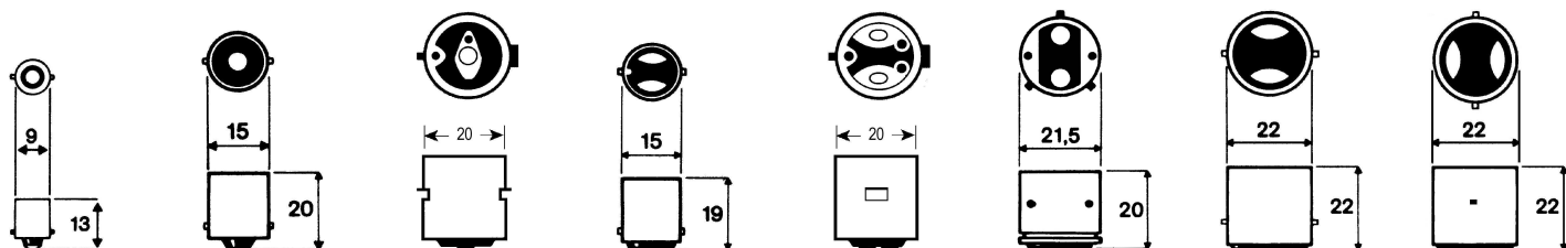
Ba9s Ba15s Ba20s Ba15d Ba20d Ba21d B22d Bx22d
